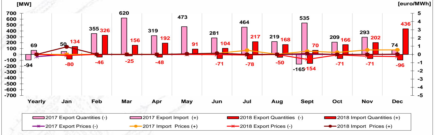
Weighted average of requested capacities correlated with auction clearing price (weighted with allocated capacities) on Ukrainian border
