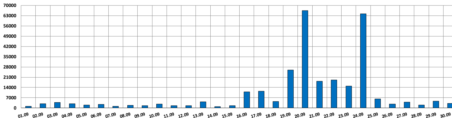
Congestion IncomeRO
